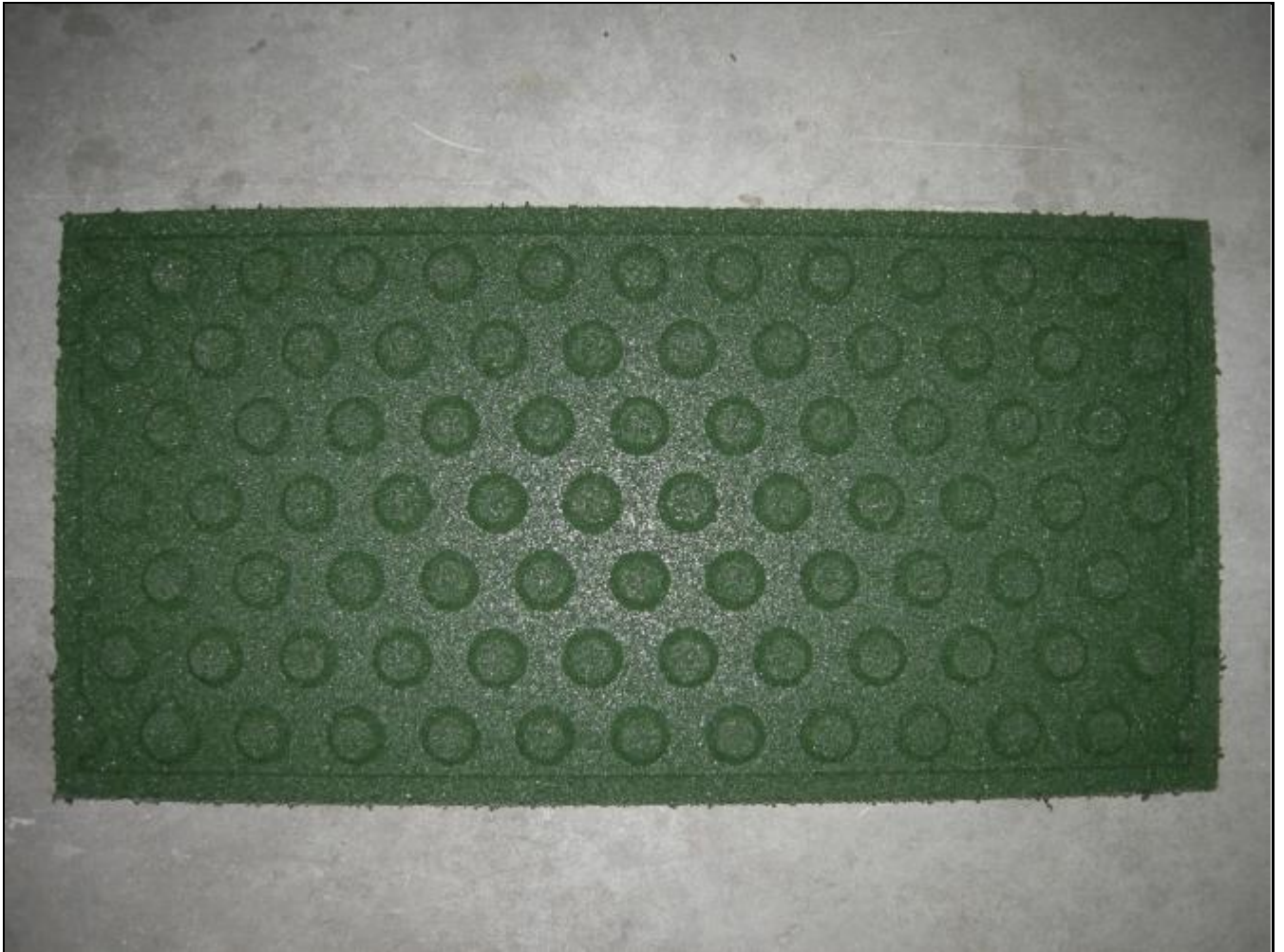
Ref. 1560. Loseta verde (1000x500x60)mm.
